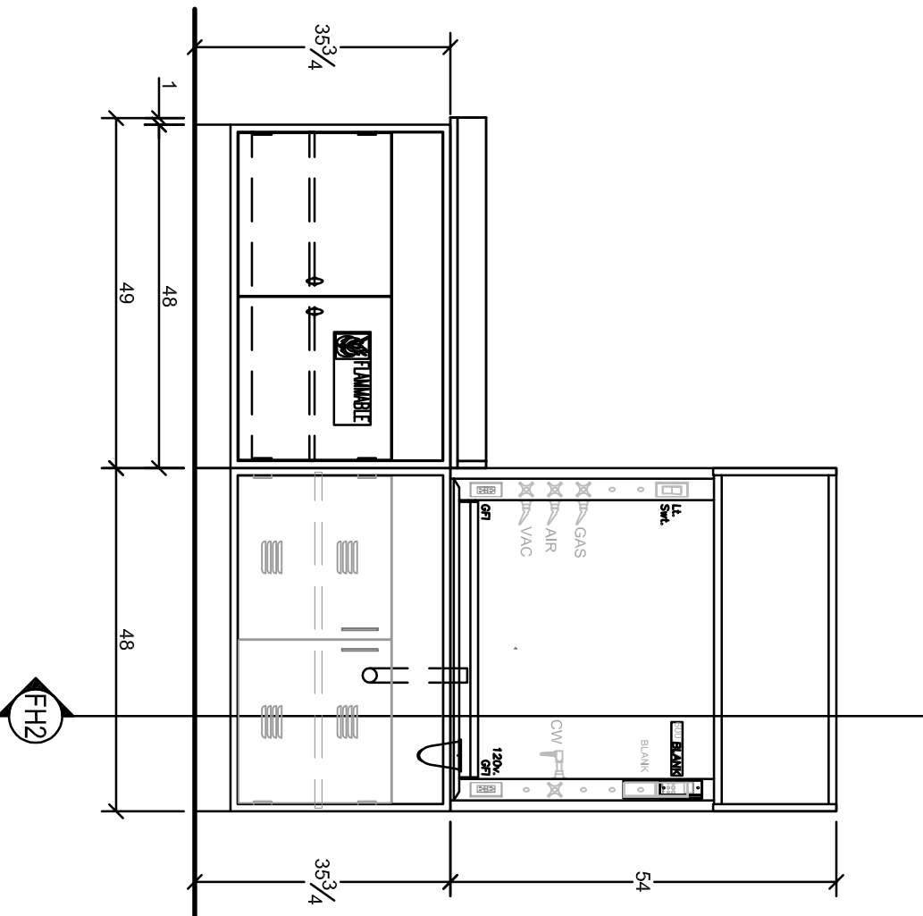
ELEVATION ROOM NO.: ROOM NAME: SCALE: 1/2" = 1'-0"
