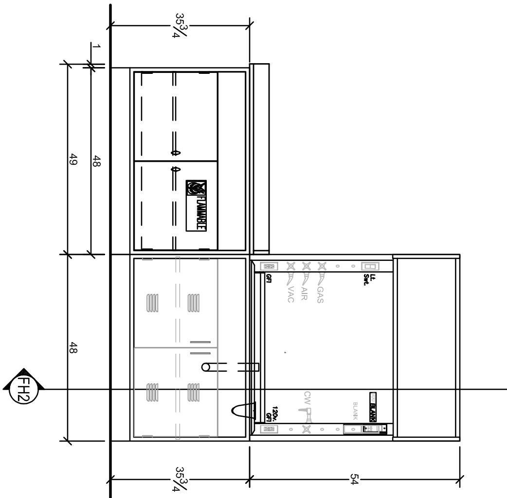
ELEVATION 09 ROOM NO: 09 ROOM NAME: PREP ROOM SCALE: 1/2" = 1'-0"
