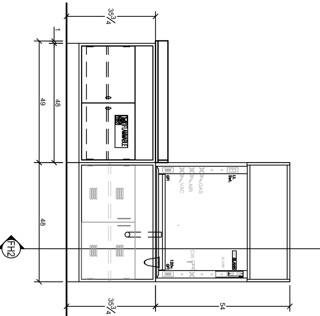
ELEVATION 09 ROOM NO. 02 ROOM NAME: PREP ROOM SCALE: 1/2" = 1'-0"
