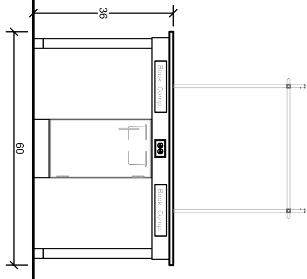
ELEVATION 14B
